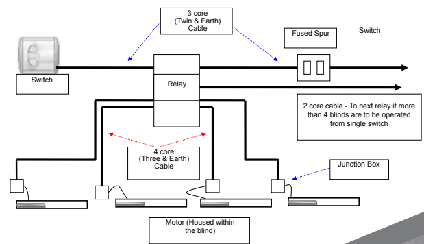
240 Volt Motorised Blinds Operating from a single hard wired Switch
